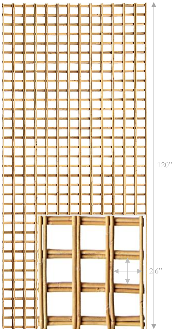
SQUARE PATTERN SKU: FP673 DOUBLE 1/2" SKIN ON; 1" OVERALL SIZES: 95-1/2"X45-1/2"; 108"X45-1/2"; 120"X45-1/2" LIST $2,000 (4X8); $2,250 (4X9); $2,500 (4X10)
