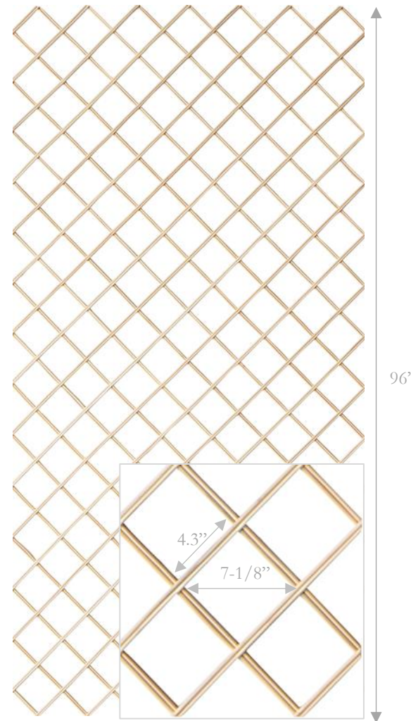
DIAMOND PATTERN SKU: FP652 DOUBLE 1/4" SKIN OFF SIZES: 122"X48; 108"X48"; 96"X48"
